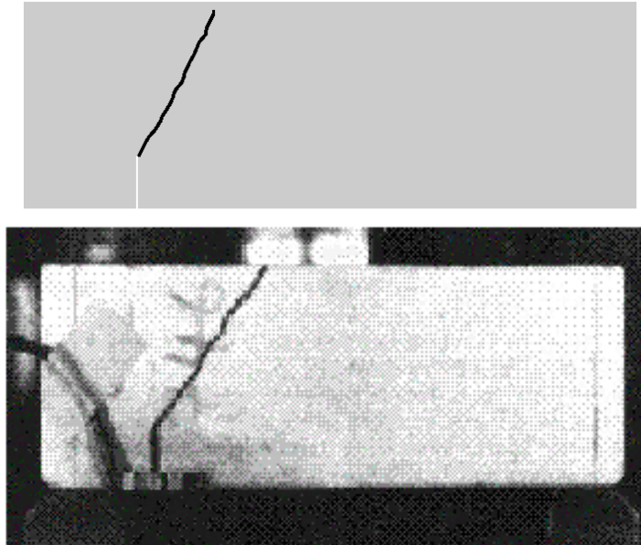
Figure 21: Comparison of the computed and observed crack pattern of the John and Shah beam under quasistatic loading
