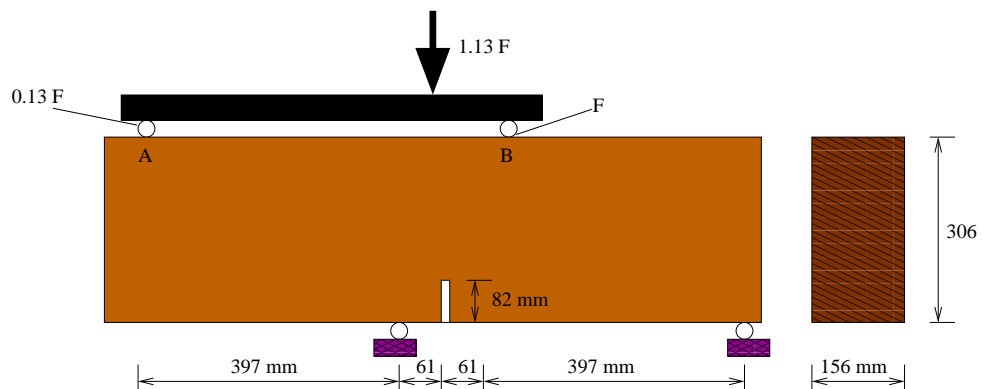
Figure 14: The tensile/shear beam from Arrea and Ingraffea
